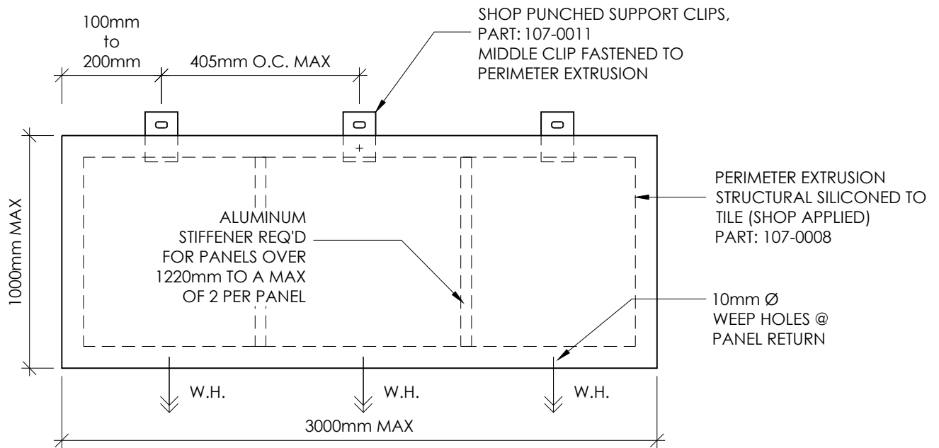
HORIZONTAL FASTENING
