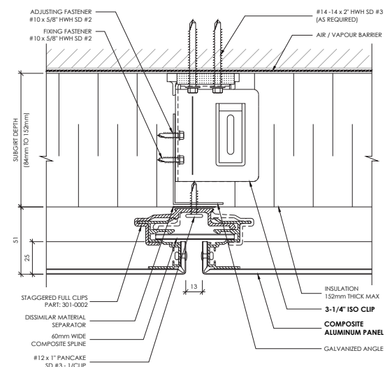
Vertical joint
