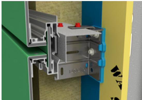
Horizontal joint
