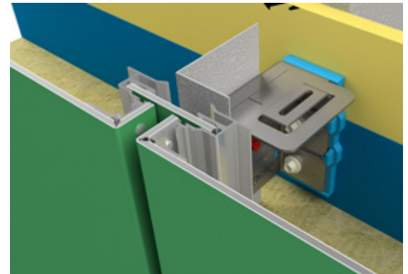
Vertical joint
